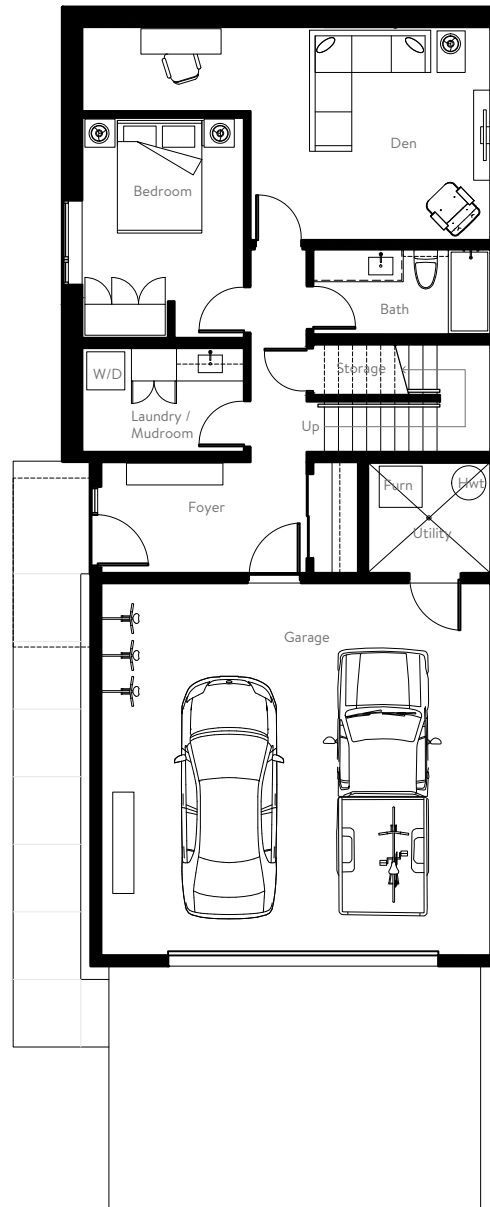
1 LEVEL 1 PLAN - UPHILL DUPLEX 1/4" = 1'-0"
